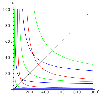
Fig. 7. The first branches of the Fuchik spectrum for the problem (29), \beta = 0.1 .
