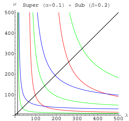
Fig. 4. Fuchik spectrum for the case super+sub, the first six pairs of branches.
