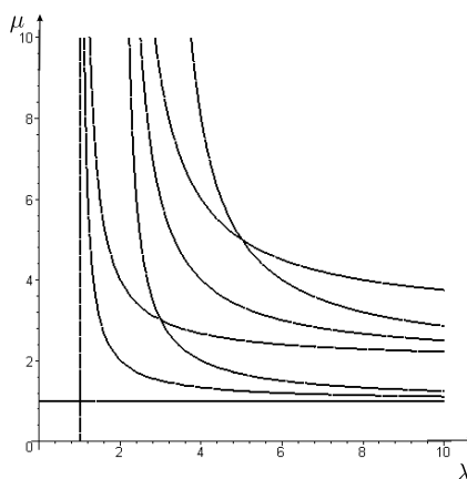
Fig. 1. Fuchik spectrum for the Dirichlet problem (4), (2).
