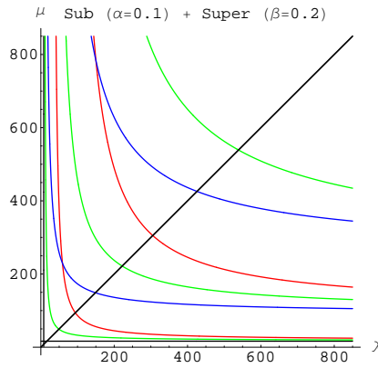
Fig. 5. Fuchik spectrum for the case sub+super, the first six pairs of branches.
