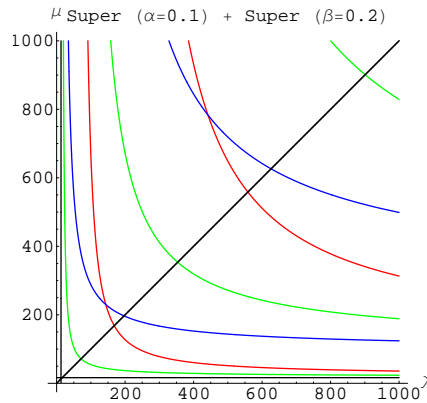
Fig. 3. Fuchik spectrum for the case super+super, the first six pairs of branches.
