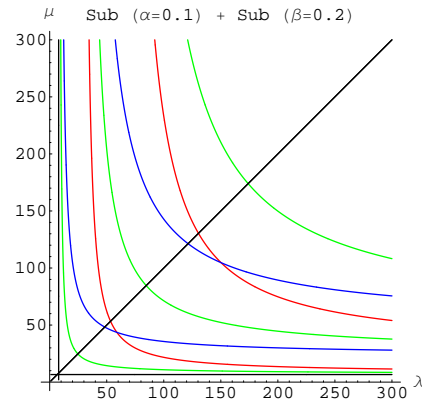
Fig. 6. Fuchik spectrum for the case sub+sub, the first six pairs of branches.
